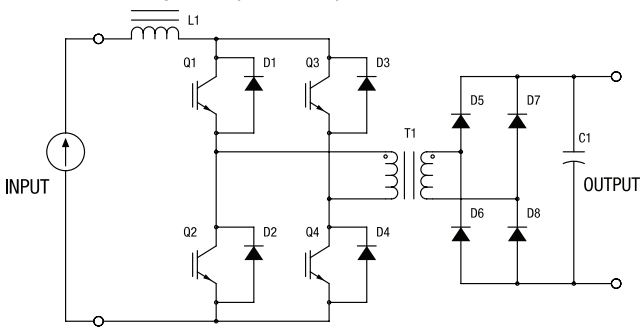
Figure 2. Current-Fed Converter
