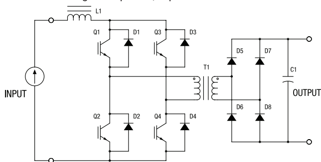
Figure 2. Current-Fed Converter
