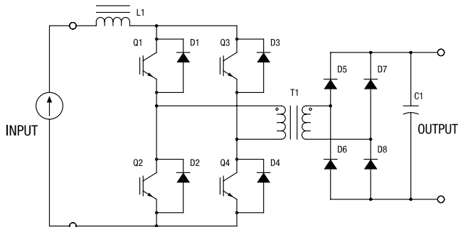
Figure 2. Current-Fed Converter
