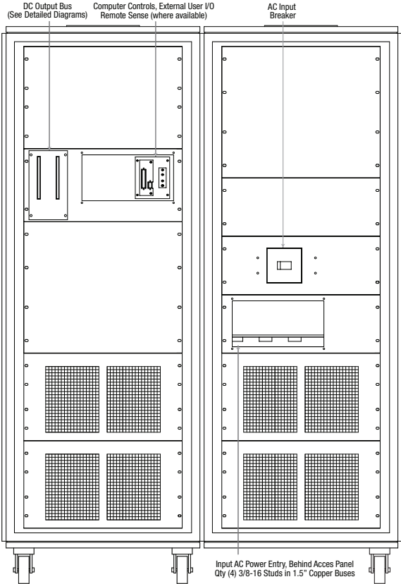
Rear Side 100 kW and 150 kW Models
