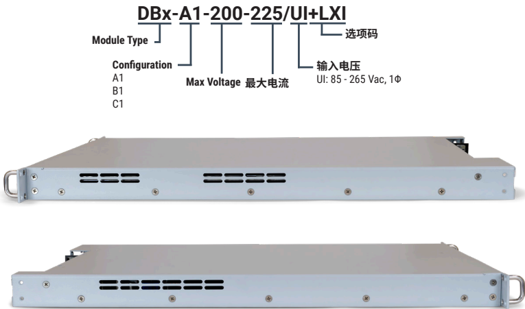
DBx Module right side view (top) and left side view (bottom)
