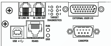
Rear communication interfaces with CANopen (+CAN) option.
