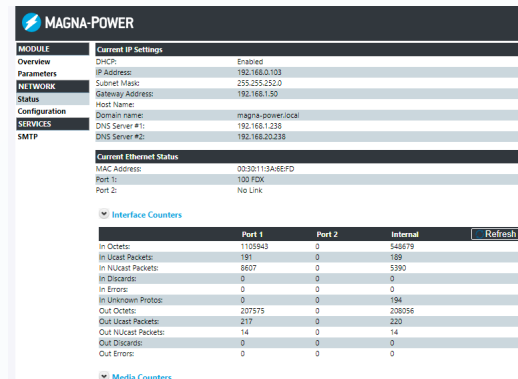
EtherNet/IP webpage hosted in Magna-Power's +EIP option with EtherNet/IP (+EIP) option.
