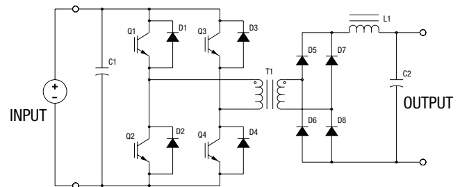
Figure 1. Voltage-Fed Converter
